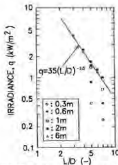
FIGURE 4 Relationship between irradiance and dimensionless distance from axis, L/D , for various sizes of heptane fires 19)
